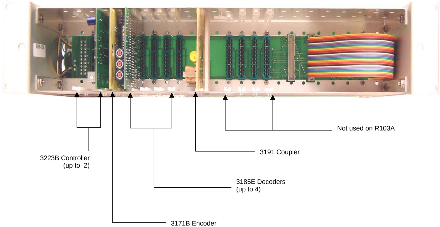
Front View – R103A (with cover removed)
